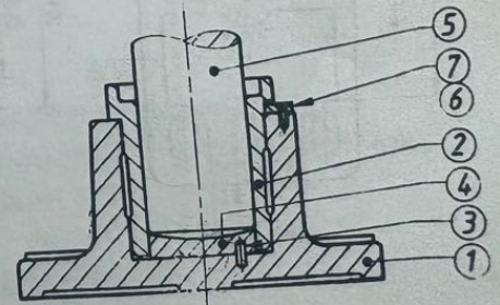
Footstep Journal Bearing Fig 20.15
